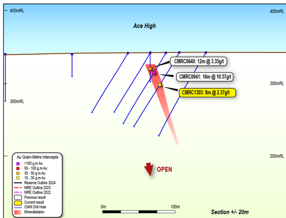
Figure 11. Ace High Section with shallow open significant broad mineralisation
