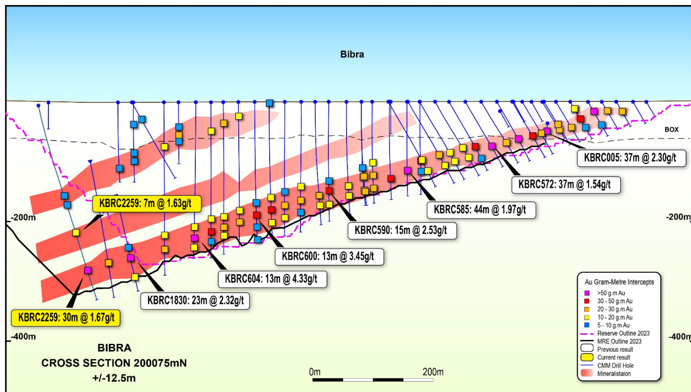
Figure 14. Bibra Section
