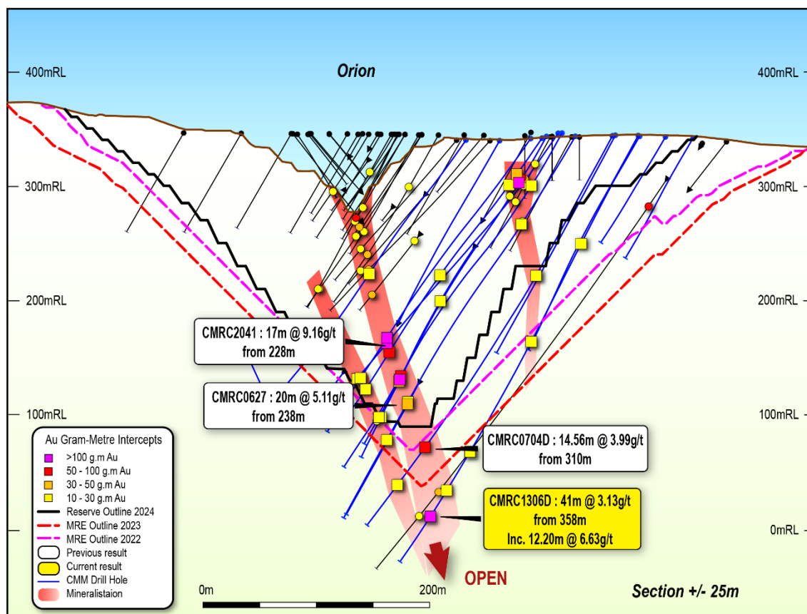
Figure 6. Orion Section with completed diamond drilling with significant mineralisation outside of the current A$1,900/oz reserve outline and A$2,300/oz resource outline.
