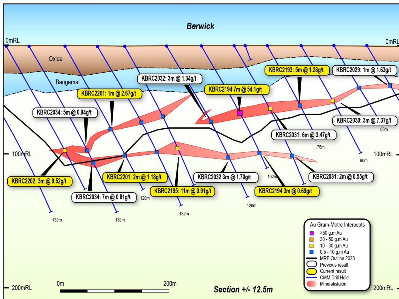
Figure 13. Berwick Section
