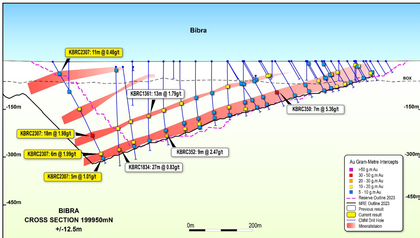
Figure 15. Bibra Section
