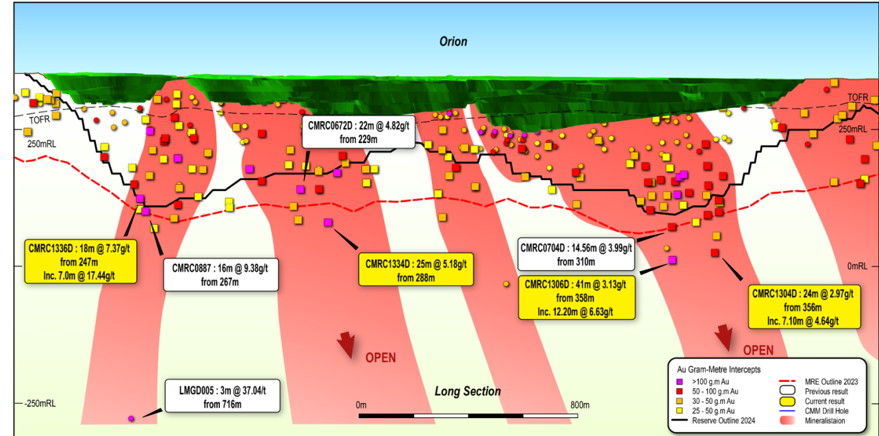
Long Section with +25-gram metre intercepts along the Orion trend looking west with significant mineralisation outside of the A$1,900/oz reserve outline and A$2,200/oz resource outline.
